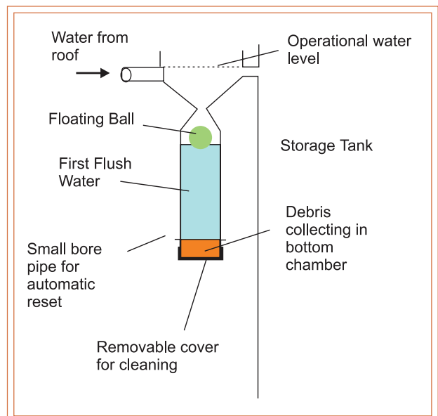
The floating ball first-flush system
