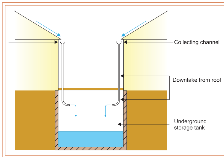
Rainwater can be stored in underground tanks as in this traditional rainwater harvesting system in Ahmedabad
