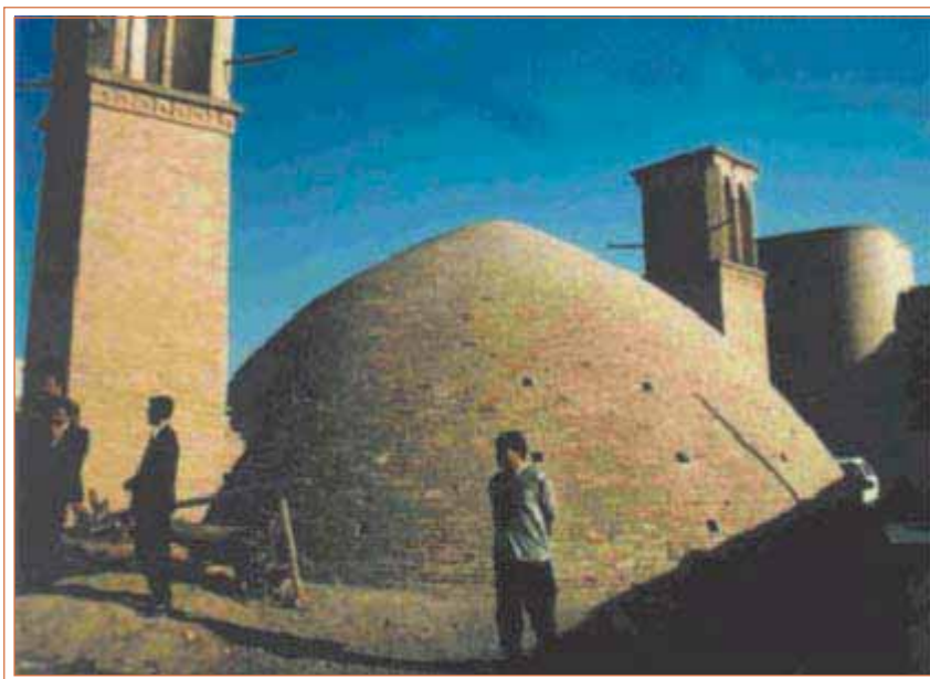
The 'Abanbar', traditional cistern in Iran (Gnadlinger) as part of a traditional rainwater catchment system for the community.
