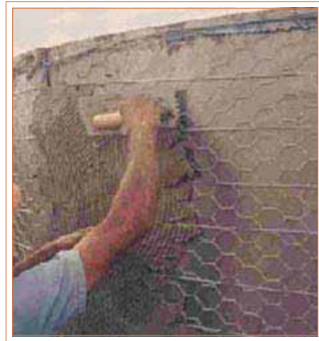
Steel sheet form wrapped by wire mesh and galvanized wire / application of first layer of mortar on top of wire (ref: Instituto Regional da Pequena Agropecuária Apropriada – IRPAA)
