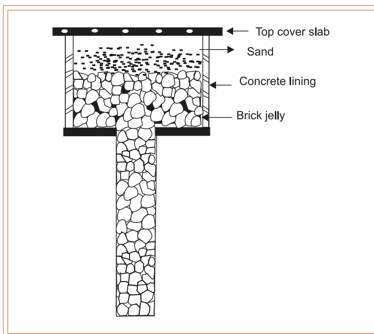
Ensuring percolation: Cross-section of percolation pit
