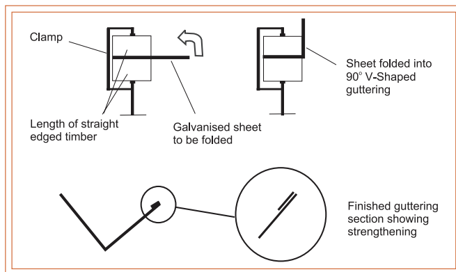
Folding galvanised steel sheet to make V-shaped guttering
