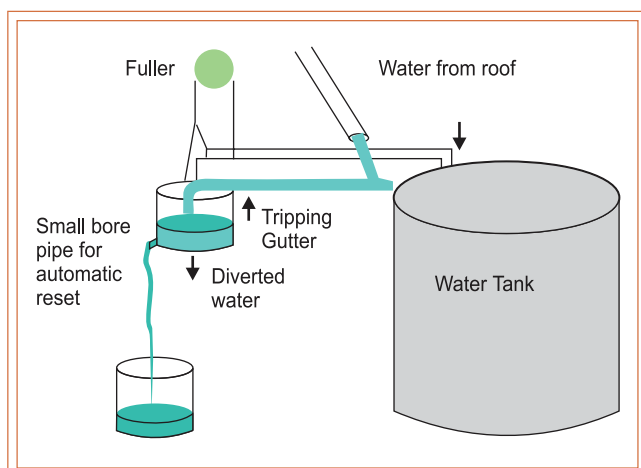
The Tripping Gutter first-flush system
