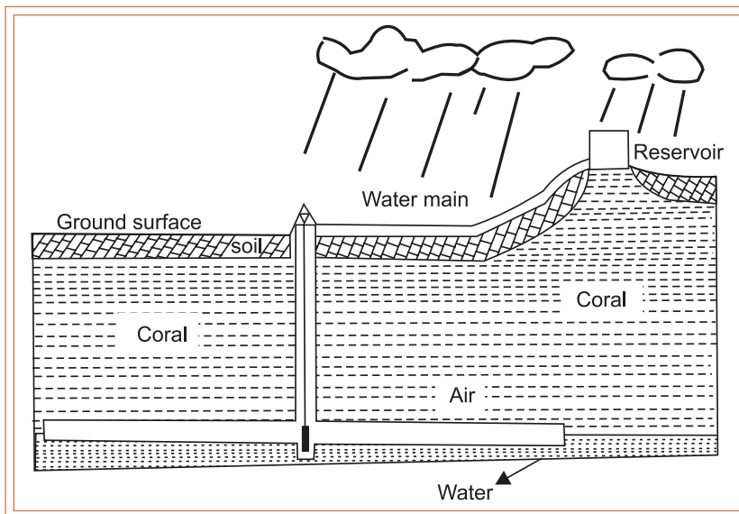
Infiltration gallery used in Barbados
