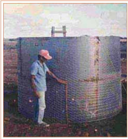
Steel sheet form wrapped by wire mesh and galvanized wire / application of first layer of mortar on top of wire (ref: Instituto Regional da Pequena Agropecuária Apropriada – IRPAA)
