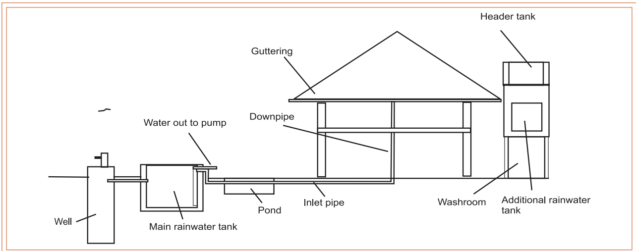
Sketch showing the whole scheme including the water tower
