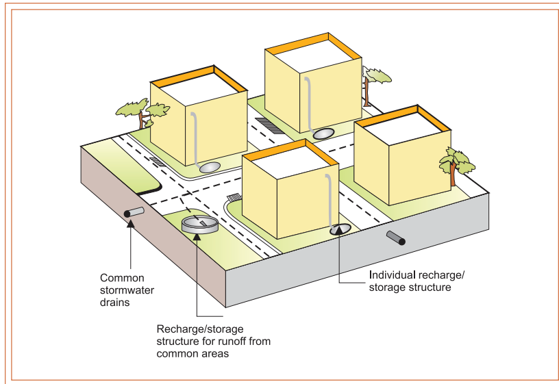
Trapping storm water drains in a community-level system
