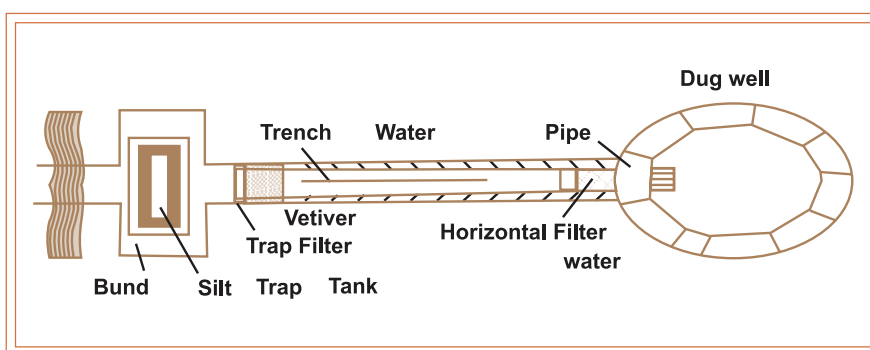
Water recharge through dug well indore method
