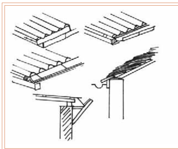
A variety of guttering types showing possible fixings
