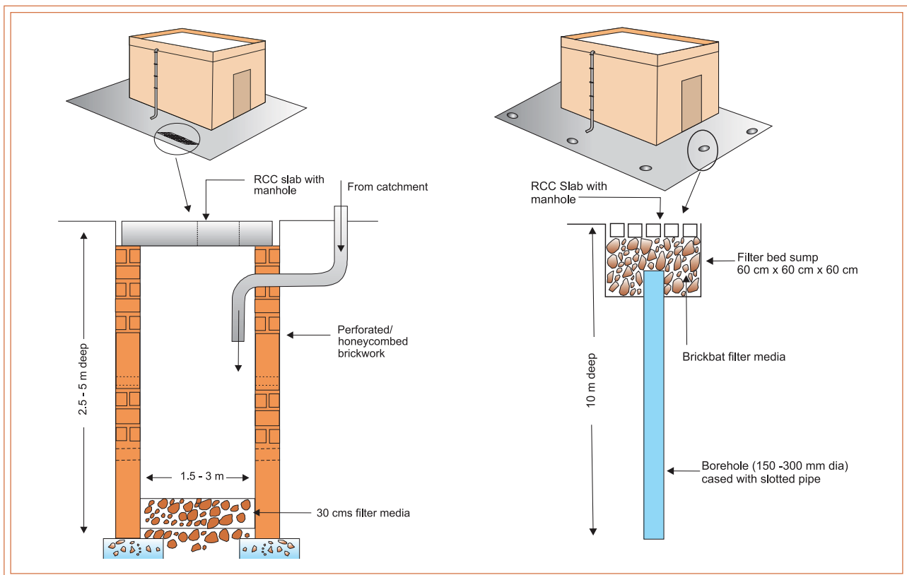
Location of recharge pit in a building area and detailed section of pit
