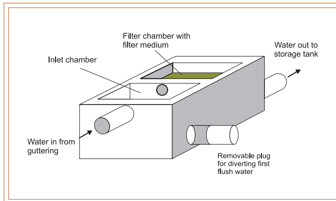
First flush device using removable plug for diverting first flush water (above) and using diversion pipe (below)
