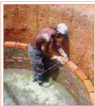
Wall construction of the tank on the concrete base
