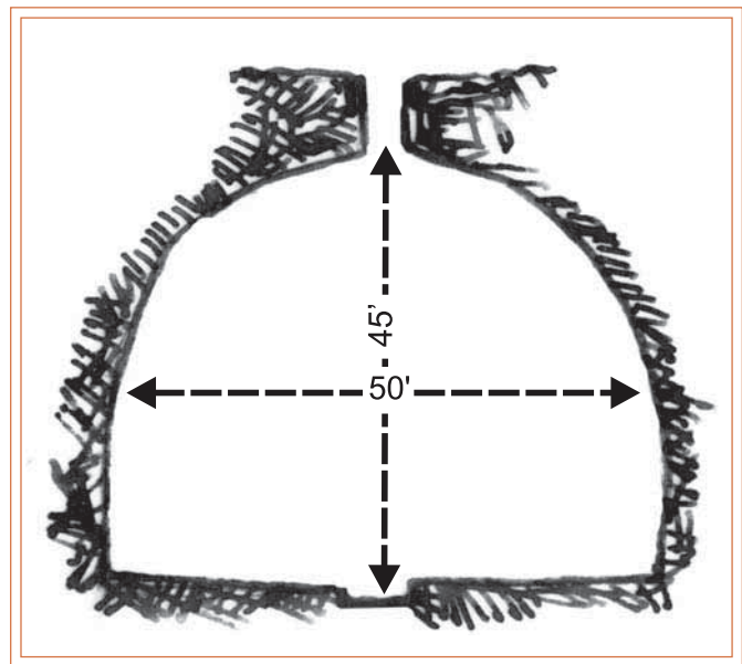
Section of cistern at Aisâwîyeh
