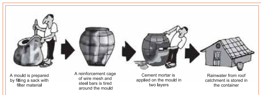
Ferrocement tanks to capture rainwater
