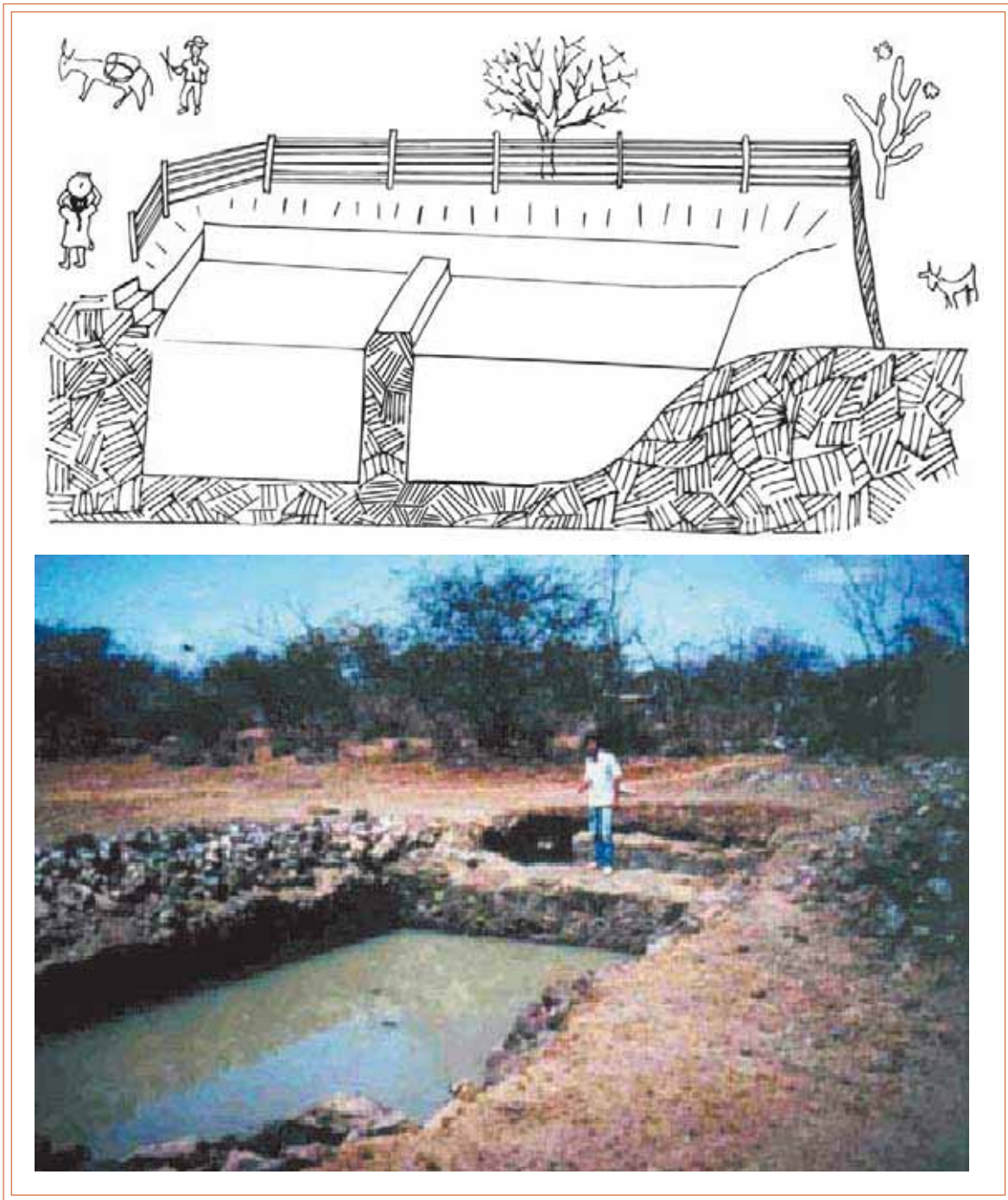
Hand dug rock cistern: In different parts of the semi-arid region there is a revival of hand-dug rock cisterns; a traditional way to harvest water for the dry season. The water is normally used for animals, but after filtering can be used for drinking purposes as well
