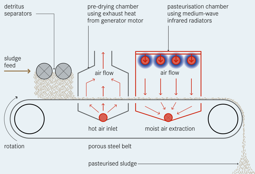
Figure 6: Schematic of the LaDePa sludge pelletizer
