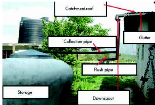
Elements of a RooftopWH system in Nepal (ICIMOD, 2009).
