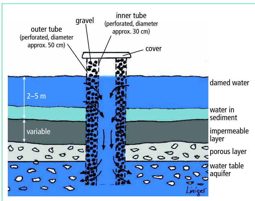
Component of a recharge well.
