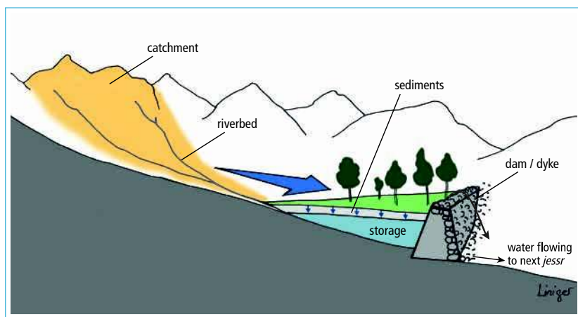
Cross-section of a jessours or warping dam system ( jessr = singular).
