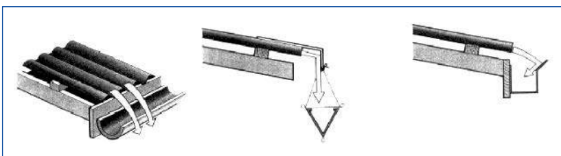
Water overshooting the gutter (left) and options to avoid water overflows (Skinner, 2003 in Doyle, 2008).
