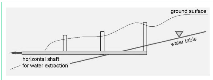
Surfacing of a foggara . (French Wikipedia)
