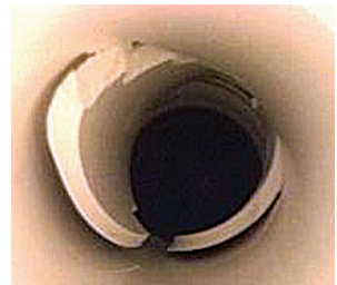
Figure 18: Casing damage as seen through a borehole CCTV camera
