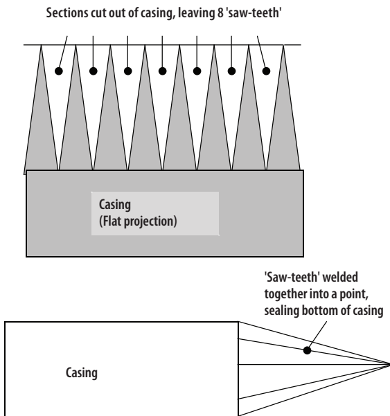
Figure 14: Sealing the bottom end of mild steel casing by the welded 'saw-teeth' method. Typical length of teeth 0.5 to 1m
