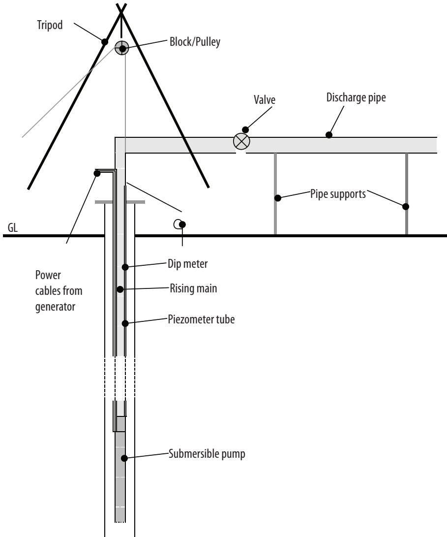
Figure 16: Typical test-pumping set-up (shown with electric submersible pump). Not to scale
