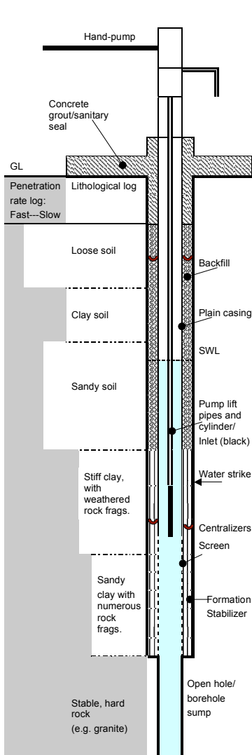
Annex 3A Borehole completion for hand-pump in a shallow, weathered zone aquifer
