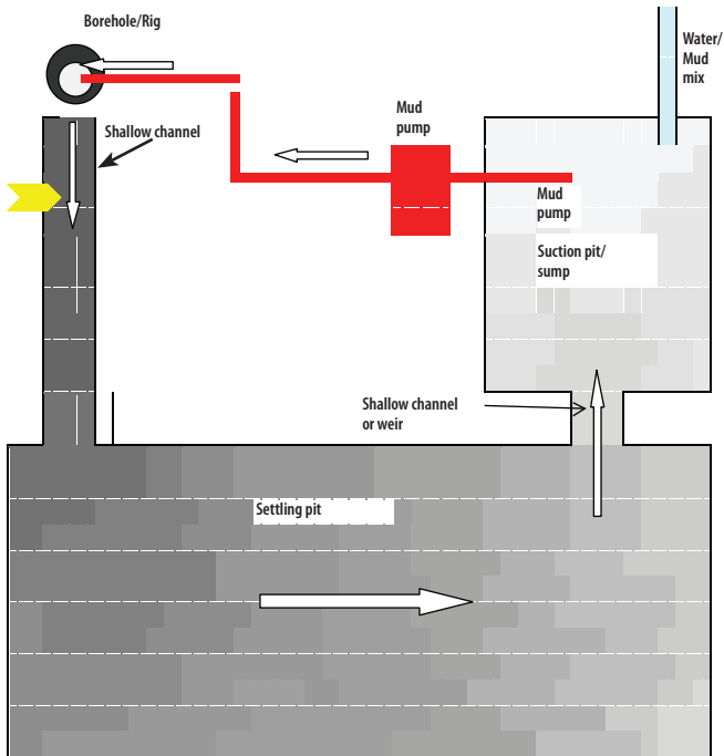
Figure 12: Schematic plan view showing mud pits and mud circulation (anti-clockwise white arrows). Not drawn to scale
