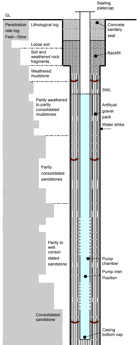
Annex 3B Borehole construction for partly consolidated sandstone aquifer (as Figure 1, hypothetical site B)
