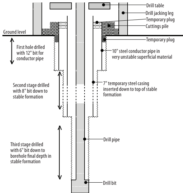
Figure 10: Schematic section of an example of temporary borehole completion. (not to scale)
