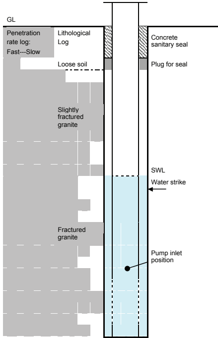
Annex 3D Borehole construction for aquifer in granite fracture zone (as Figure 1, hypothetical site D)
