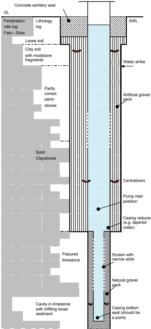
Annex 3C Borehole construction for combined sandstone and limestone aquifers (as Figure 1, hypothetical site C)
