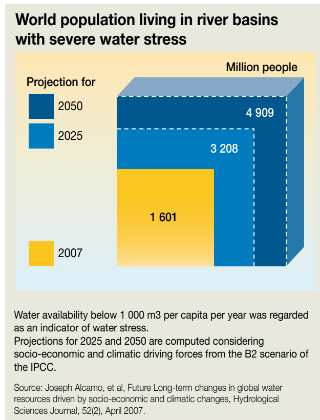
Figure 21: Increasing water scarcity with population increase.
