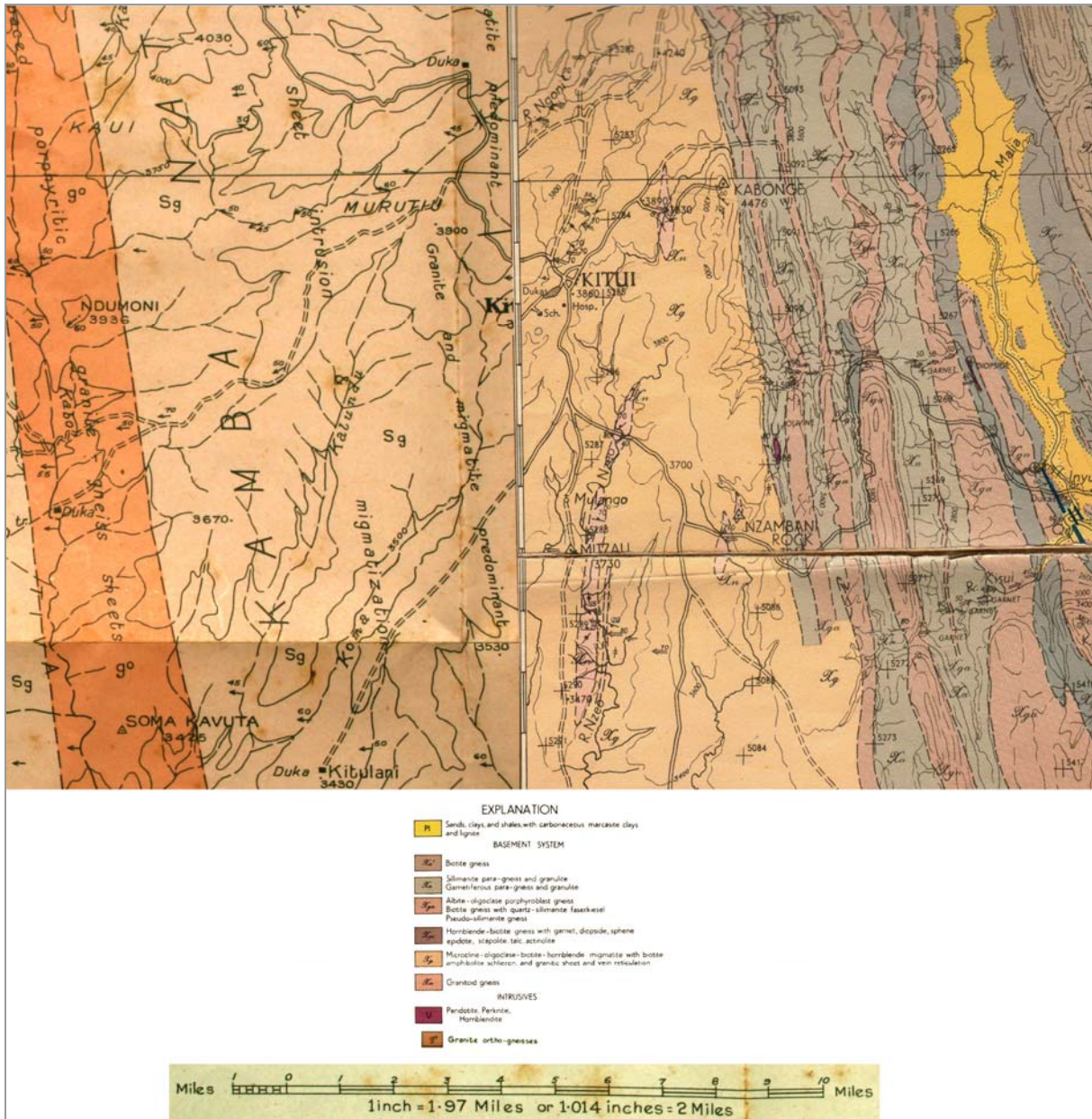
Combined geological map after Schoeman (1948, left) and Sanders (1954, right)
