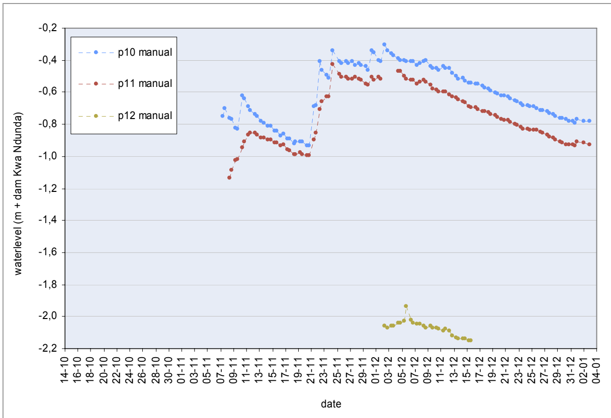
Piezometers next to dam Kwa Ndunda
