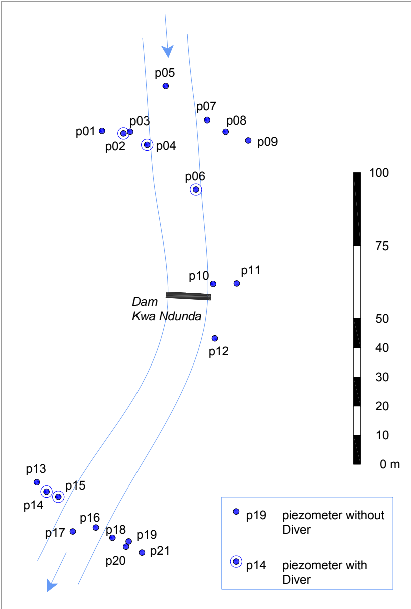
Figure 3.5 Overview of piezometers
