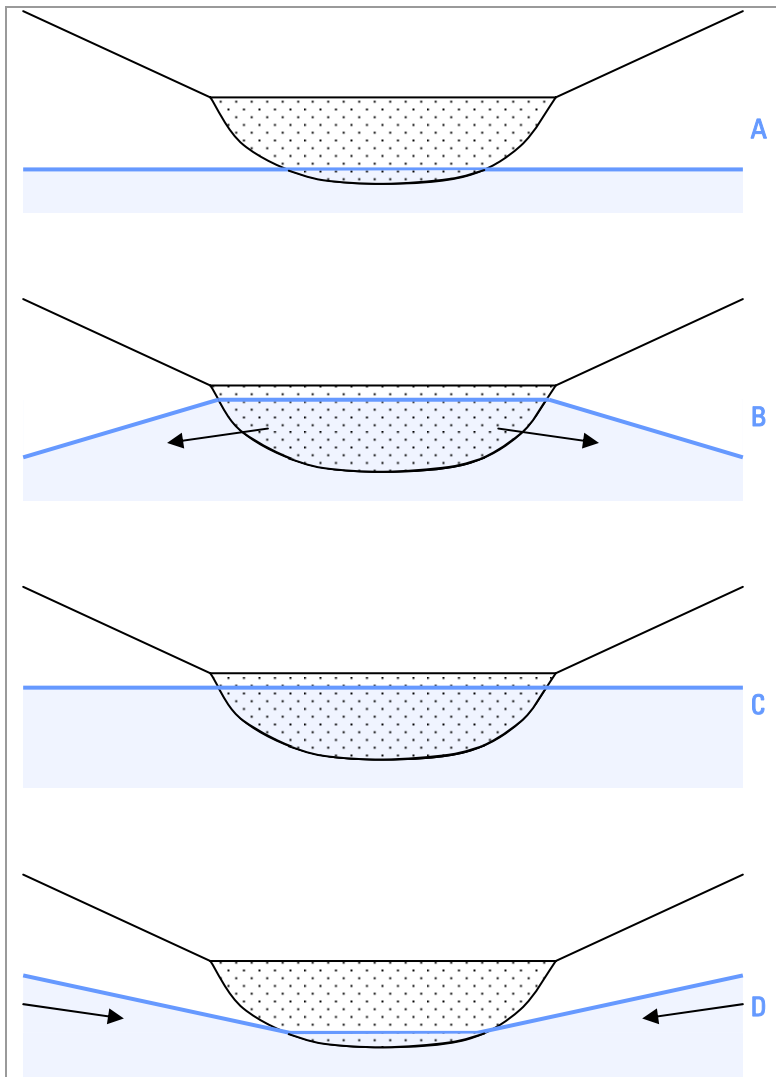
Figure 5.9 Schematic cross-sections over the riverbed: low water level (A), recharge from the riverbed to the banks (B), high water level (C) and recharge from the banks to the riverbed (D).
