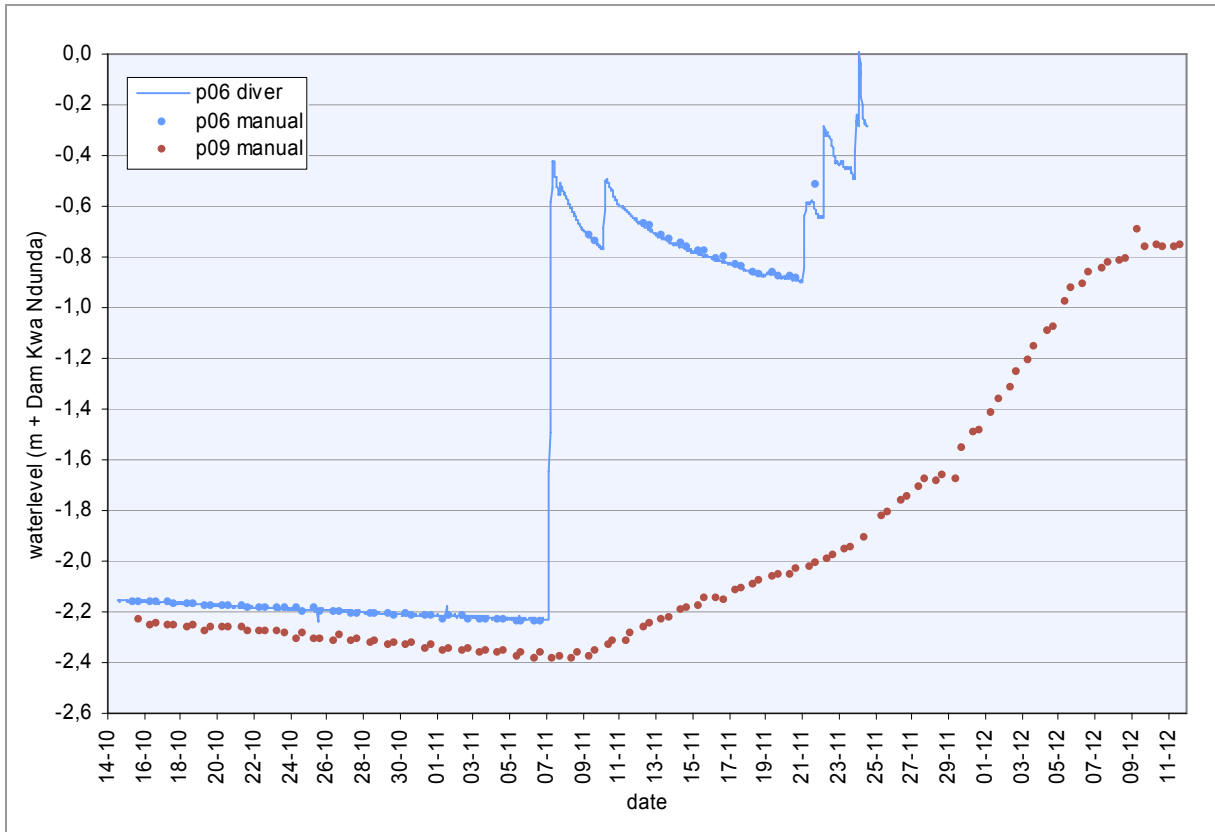
Figure 4.23 Water level in the riverbed and the riverbank (p06 and p09)
