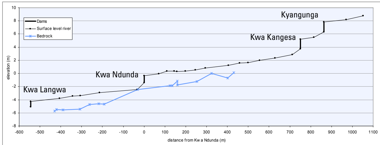
Figure 4.17 Longitudinal profile of the surface level of the river and the hardrock
