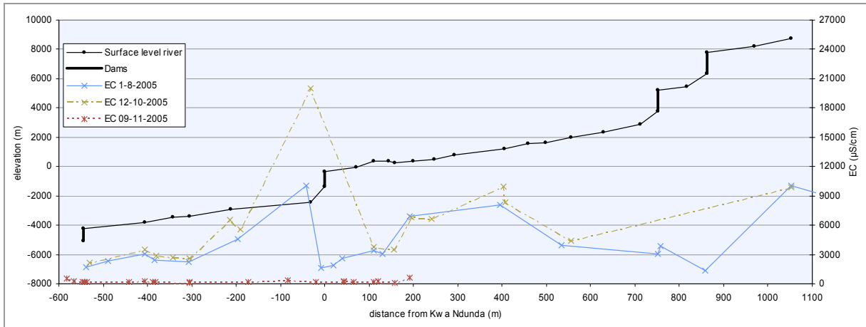
Figure 4.27 Longitudinal profile with EC
