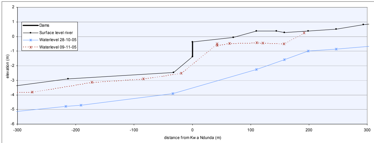
Figure 4.21 Detail of the step change in water levels around dam Kwa Ndunda
