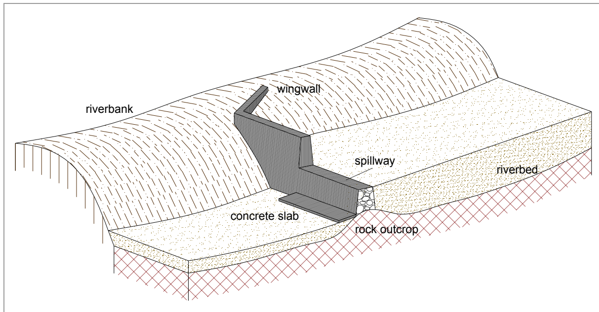
Figure 2.26 The different aspects of an effective sand storage dam
