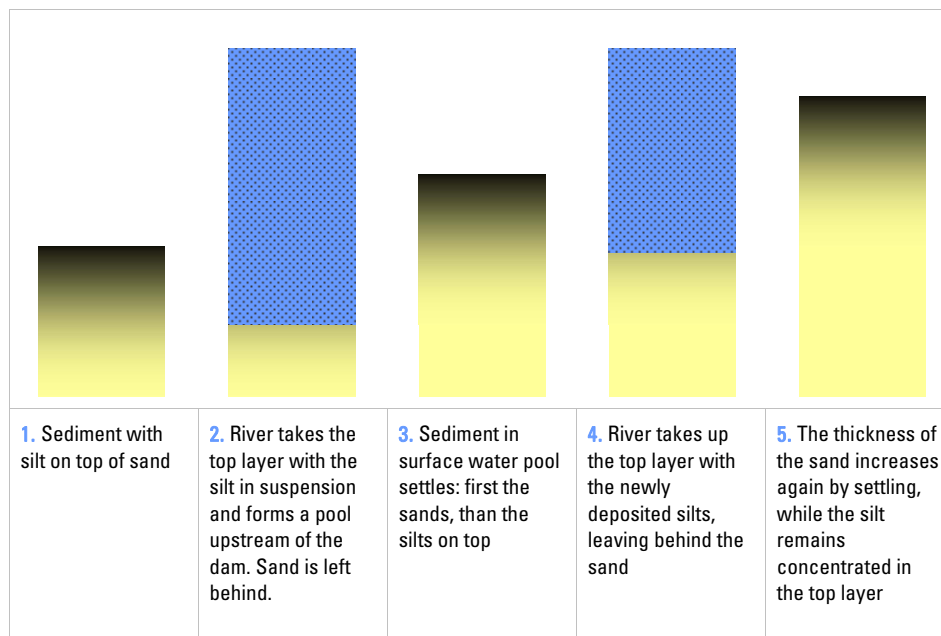
Figure 5.3 The process of sedimentation upstream of a sand storage dam
