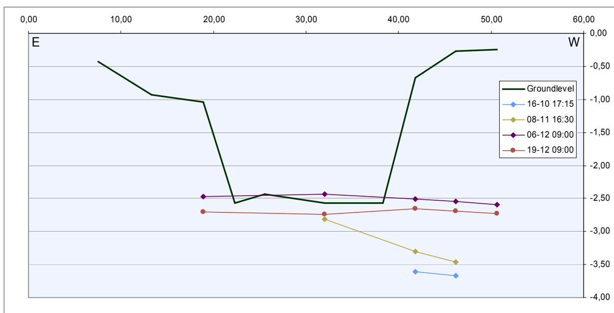
Figure 4.26 Downstream cross-section with changing water levels in time
