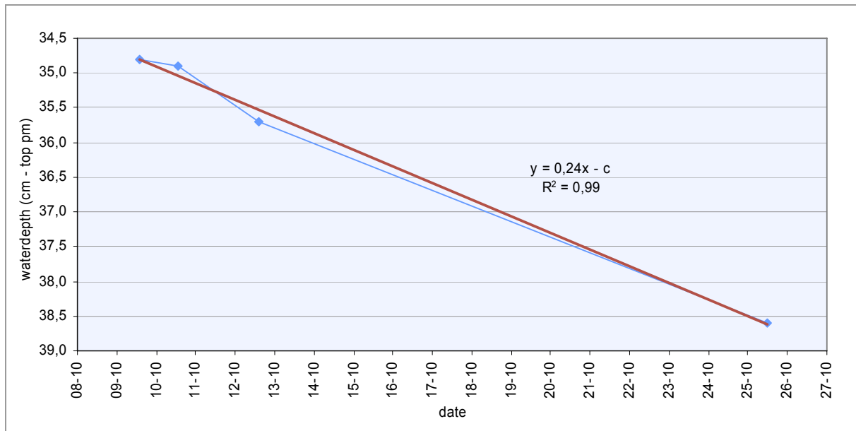
Figure 4.12 Observed evaporation in the sub-surface evaporation pan
