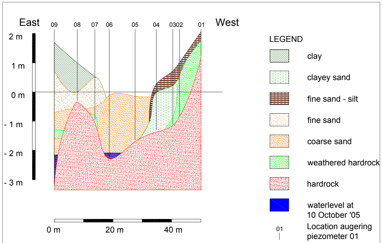
Figure 4.13 Upstream cross-section. The direction of sight is downstream
