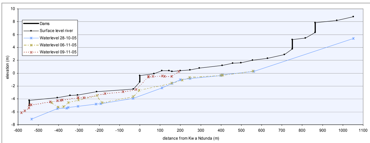
Figure 4.20 Longitudinal profile with changing water levels
