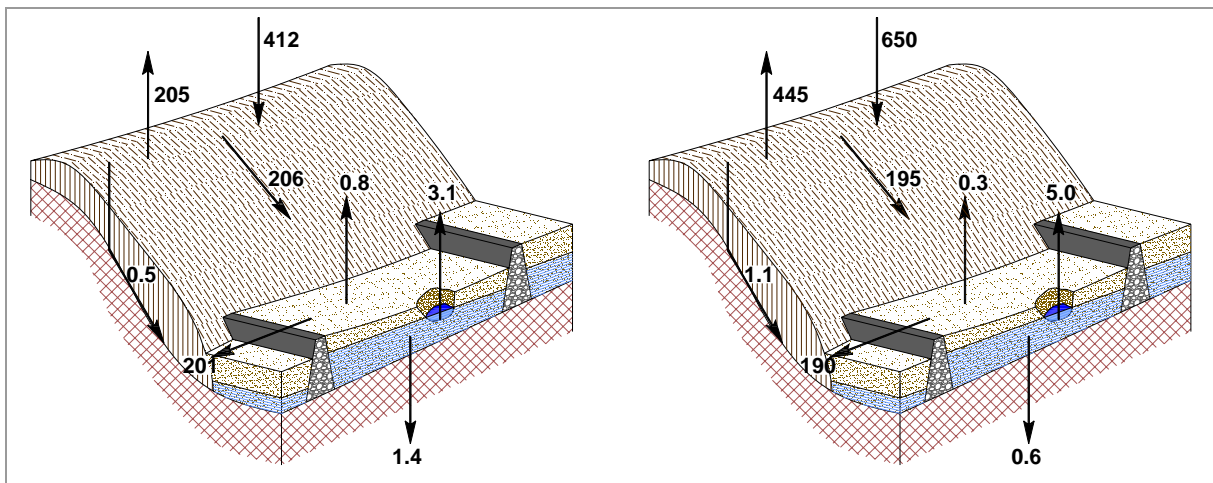
Figure 5.14 Water balances for the season March to October (left) and November to February (right); values in thousands of m 3 per season
