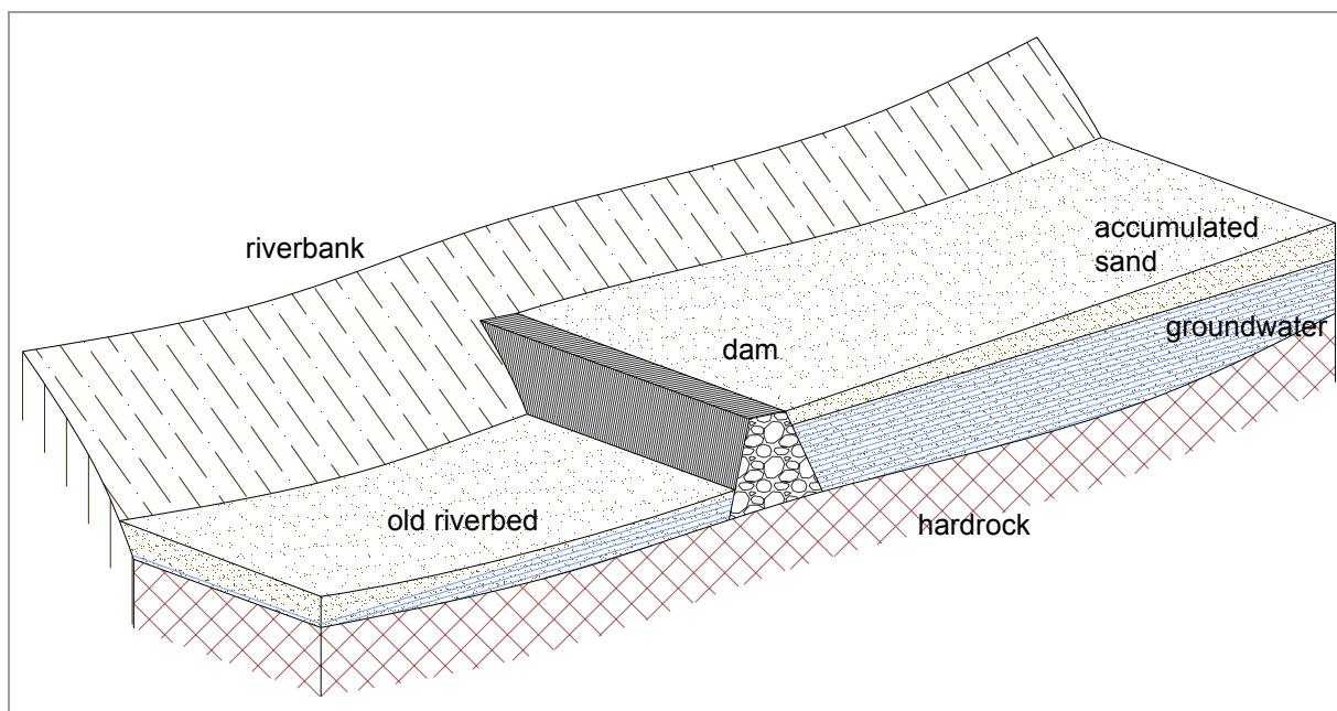
Figure 2.23 Principle of a sand storage dam
