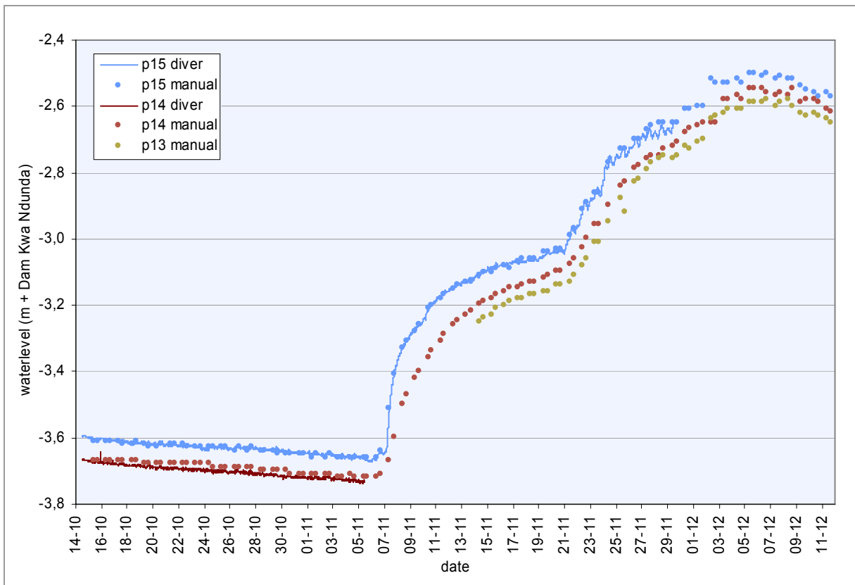
Figure 4.24 Water level in the riverbanks
