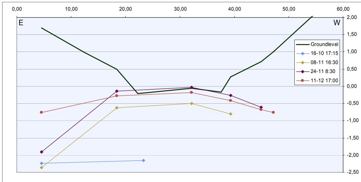
Figure 4.25 Upstream cross-section with changing water levels in time
