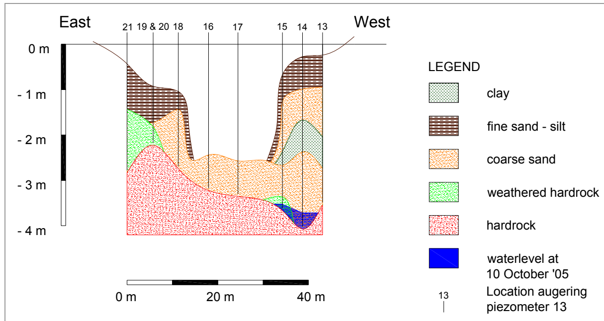
Figure 4.14 Downstream cross-section. The direction of sight is downstream
