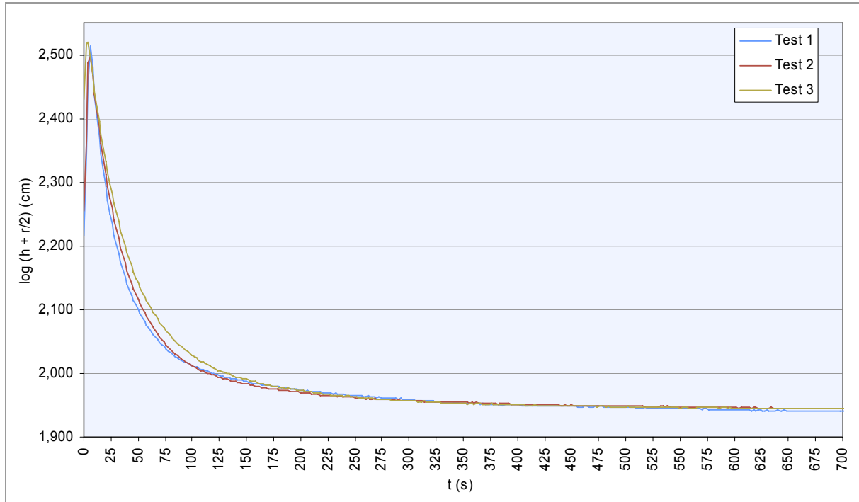
Figure 4.15 Results from inversed auger hole tests in piezometer 15
