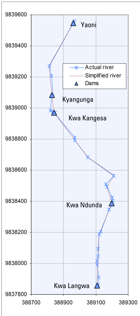
Figure 4.16 Actual and simplified path of river (UTM coordinates)
