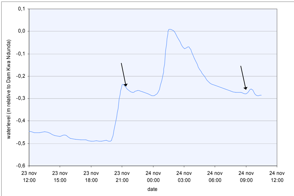
Figure 4.31 Water level in piezometer 6 at 23 and 24 November, on which discharge estimates were made. The arrows indicate the moments of discharge estimates
