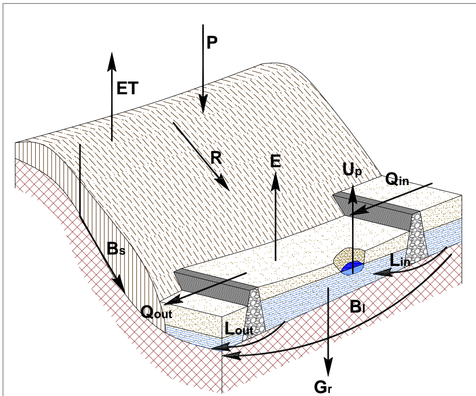
Figure 5.11 Schematic water balance of the sand storage dam
