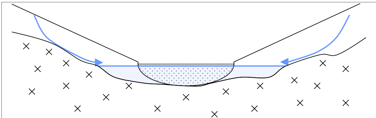
Figure 5.8 Schematic cross-section with lateral baseflow
